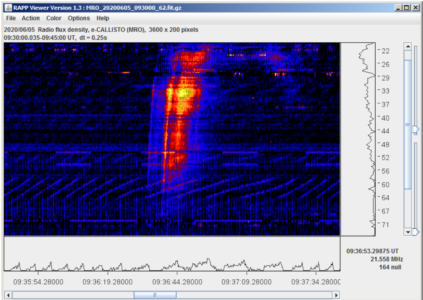
Fig. 3: Probably the first observation of a burst with Callisto, heterodyne up-converter and LWA at Metsähovi Radio Observatory (MRO) in Finland.
