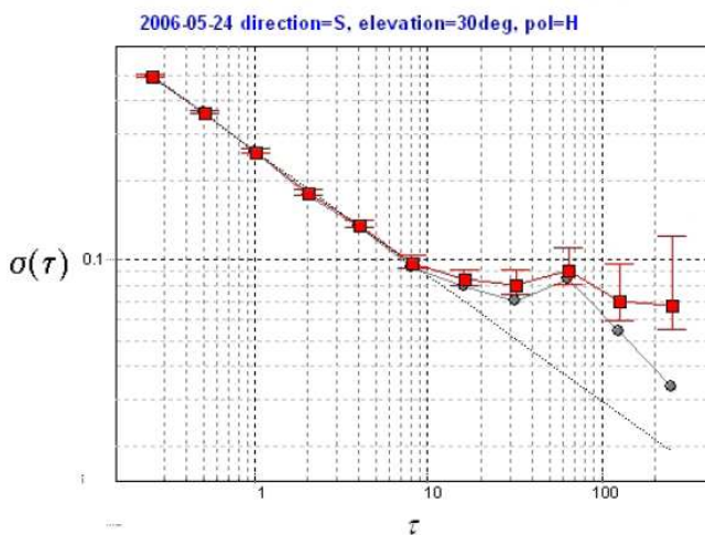
Fig. 25. Allan-time and Allan-variance of horizontal polarized spectral line at 410.22MHz measured at Humain station.
