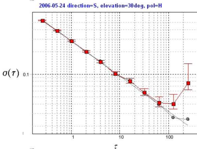
Fig. 24. Allan-time and Allan-variance of horizontal polarized spectral line at 244.19MHz measured at Humain station.
