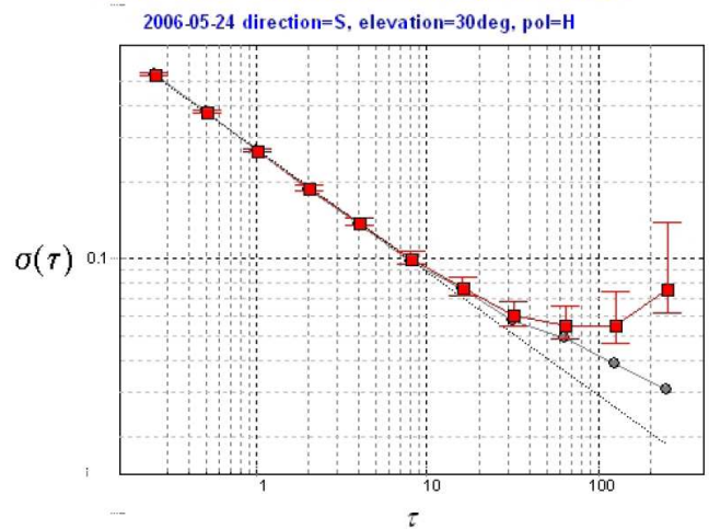
Fig. 26. Allan-time and Allan-variance of horizontal polarized spectral line at 607.19MHz and measured at Humain station.
