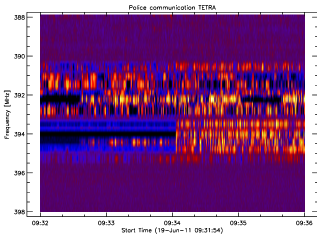
Fig. 36. TETRA, permanent communication 24h/7d in digital broad-band transmission.
