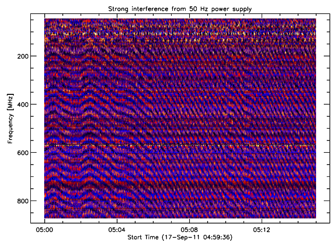
Fig. 52. Wobbling cords (50 Hz) due to a cheap, overloaded power supply.
