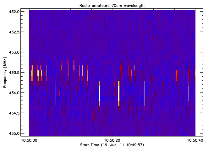
Fig. 37. Sporadic narrow frequency modulation (NFM) from amateur radio communication (HAM) in 70 cm band.
