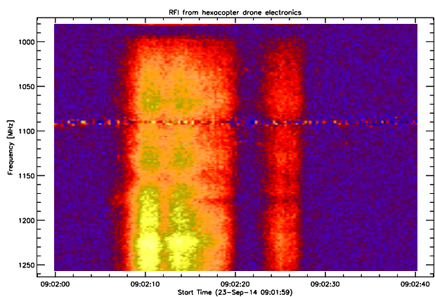
Fig. 46. Hexacopter drone flying above the 5 m dish at Bleien observatory Switzerland. The high current electronics produces broad band RFI.
