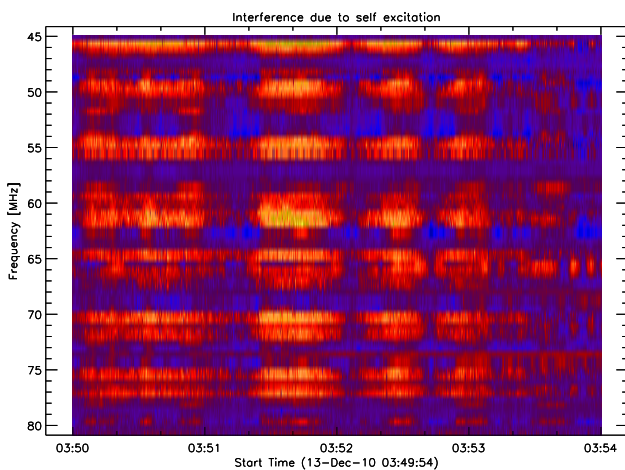
Fig. 50. Self excited system due to bad shielding and high gain amplifier.
