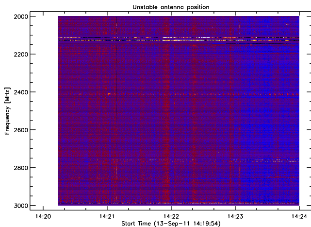
Fig. 51. Flux fluctuations (vertical stripes) in the S-band observed at Bleien observatory Switzerland with FFT-spectrometer Phoenix-3.
