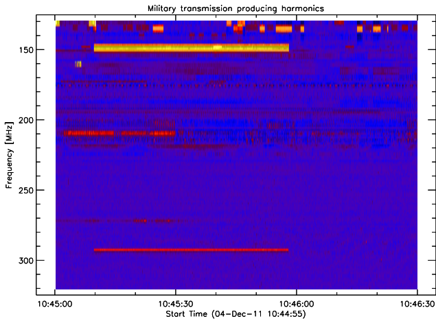
Fig. 32. Nearby military transmission around 147 MHz producing 1st harmonics at 294 MHz.
