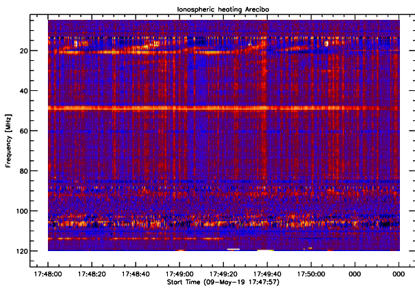
Fig. 58. Interference due to ionospheric heating at Arecibo Observatory.
