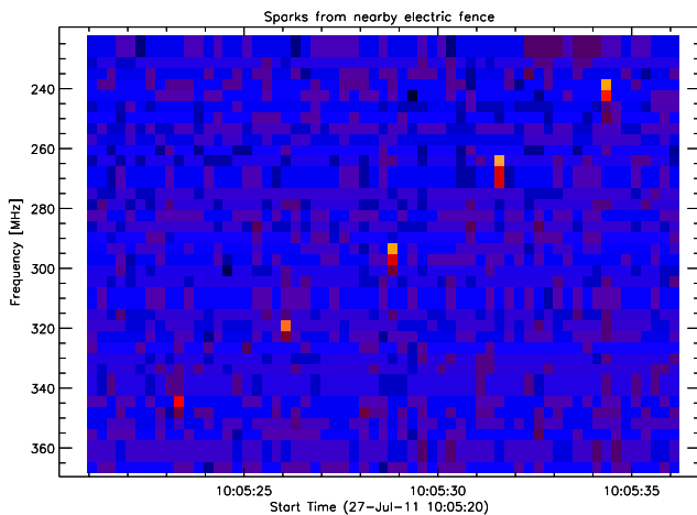
Fig. 20. Interference due to electric fence near the telescope observed at Bleien observatory, Switzerland. Antenna = parabolic dish 7 m, linearly polarized 45^\circ .
