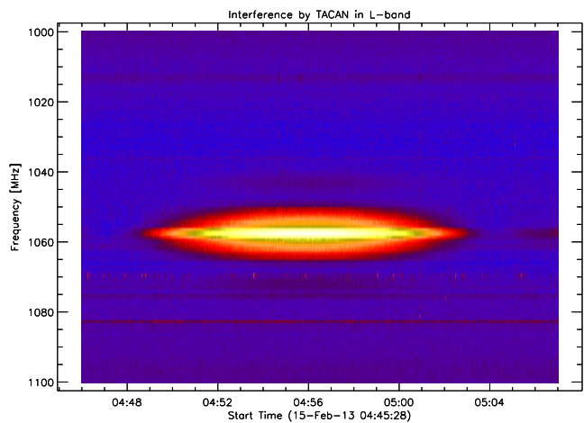
Fig. 44. TACAN signal from aircraft at 1057 MHz observed with Callisto on a 5 m dish at Bleien observatory Switzerland.
