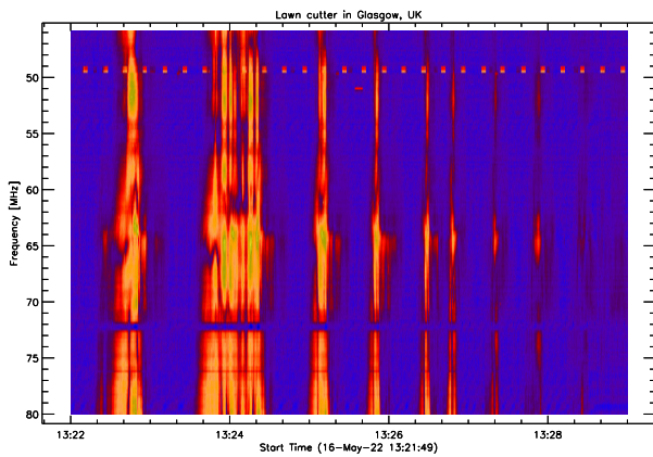
Fig. 47. Lawn cutter at observatory of University of Glasgow, UK. The strong current of drive electronics produces broad band RFI.
