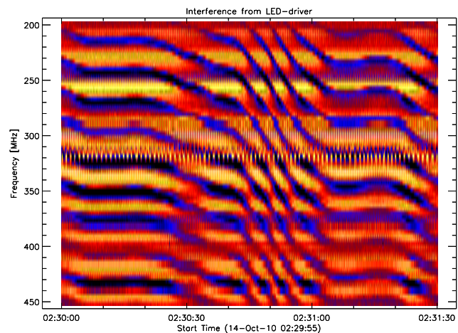
Fig. 23. Interference due to LED-driver circuit near the telescope observed at Metsähovi observatory, Finland. Antenna = log-per DVB-T like, linearly polarized.
