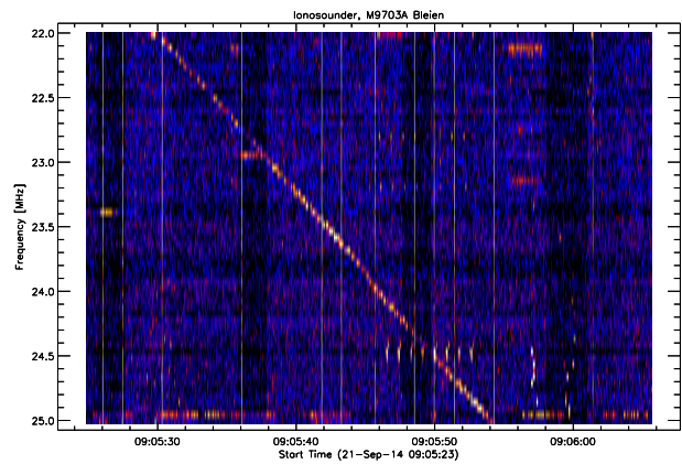
Fig. 45. Shortwave ionosonde observed with Long Wavelength Antenna (LWA) at Bleien observatory in Switzerland.
