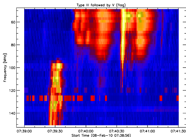
Fig. 8. Type V solar radio burst observed at Ooty observatory, India. Antenna = home made, linearly polarized, pointing to zenith.
