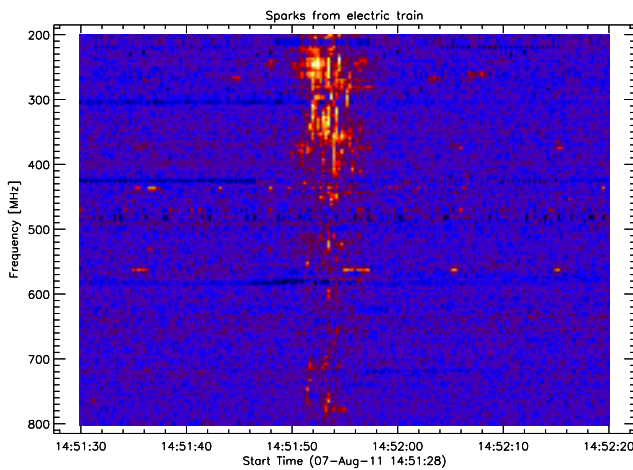
Fig. 25. Quasi burst caused by a nearby electric train of Südostbahn(SOB). Antenna = log-per, linearly polarized.
