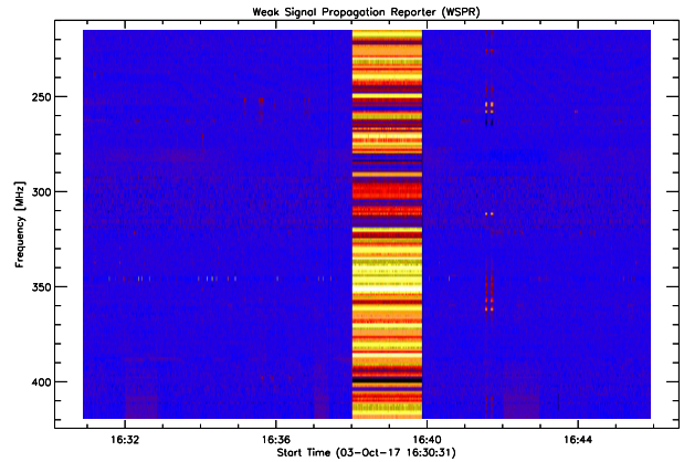
Fig. 57. Interference generated by a WSPR transmission.
