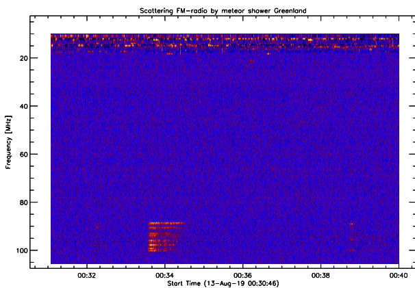
Fig. 60. Interference due to scattered FM-radio on meteor shower.
