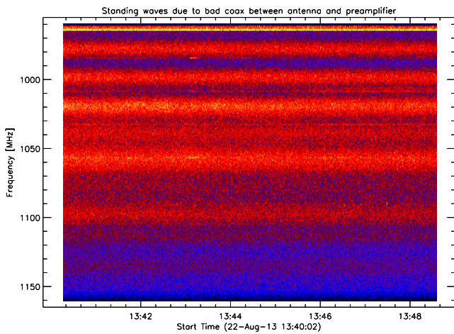
Fig. 54. Interference introduced by unmatched components in the high frequency path standing waves (SW).
