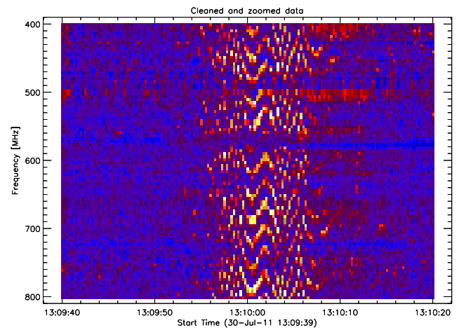
Fig. 26. Necklace burst man made by a motor cycle. Antenna = log-per, linearly polarized.
