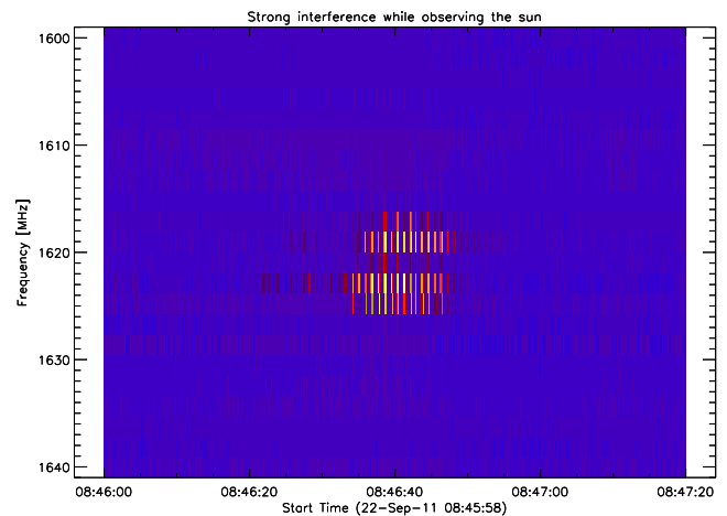
Fig. 41. Fast moving IRIDIUM satellite in the L-band near 1620 MHz observed at Bleien observatory Switzerland.
