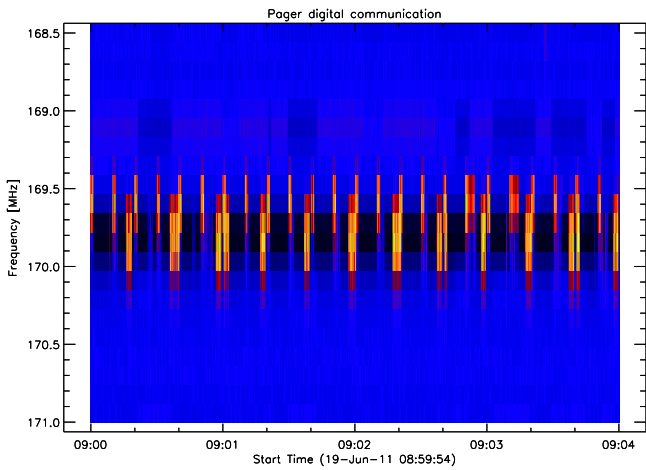
Fig. 33. Permanent communication in narrow band frequency shift keying (NFM-FSK).
