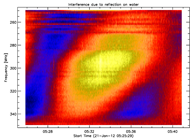
Fig. 15. Interference due to reflection of the solar radiation on the surface of a sea. Antenna = group of 4x4 Yagis at Crimea island Ukraine, linearly polarized, pointing to sunrise.
