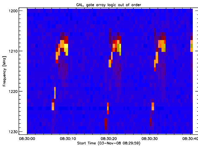
Fig. 21. Interference due to damaged gate array logic in the front-end of the telescope observed at Bleien observatory, Switzerland. Antenna = parabolic dish 5 m, linearly polarized 45^\circ .
