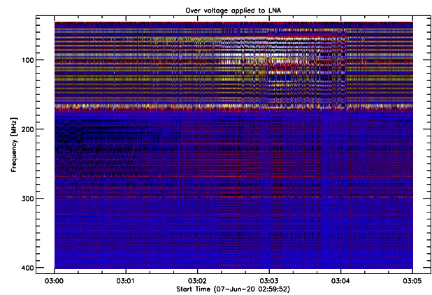
Fig. 62. Very strong interference due to too high voltage supply of the LNA.
