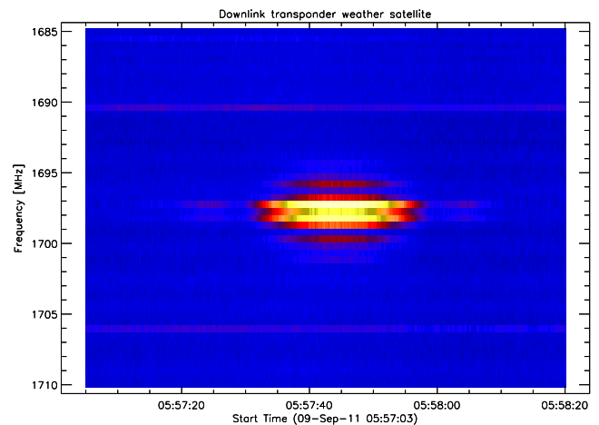
Fig. 42. Fast moving weather satellite in the L-band near 1697 MHz observed at Bleien observatory Switzerland .
