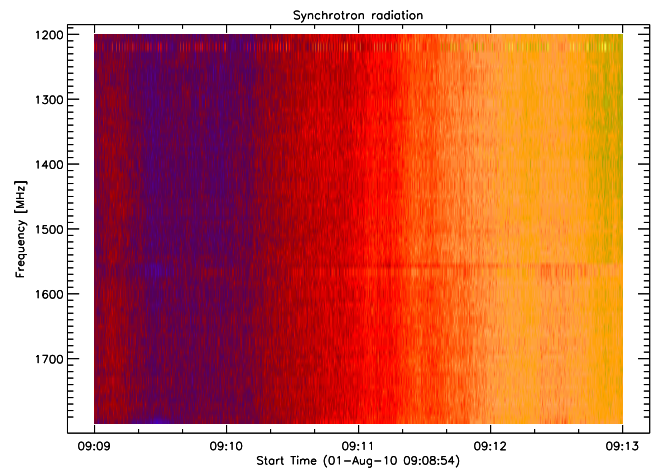
Fig. 12. Gyro-synchrotron solar radio radiation observed in L-band at Bleien observatory, Switzerland. Antenna = 5 m dish, linearly polarized, pointing to sun.
