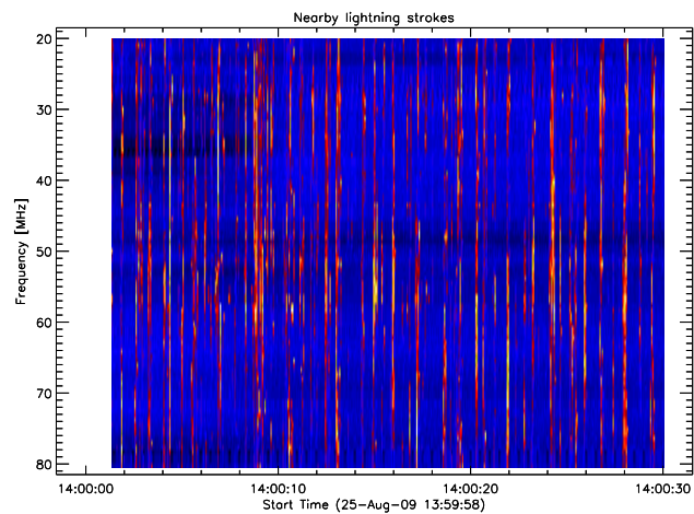
Fig. 16. Broad band radiation generated by nearby lightning strokes observed at Bleien observatory, Switzerland. Antenna = biconical dipole, linearly polarized.
