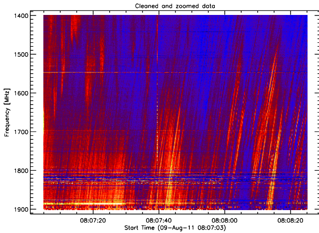
Fig. 11. DCIM (decimetric microwave) solar radio flare with fiber structures observed at Bleien observatory, Switzerland. Antenna = 5 m dish, pointing to sun.
