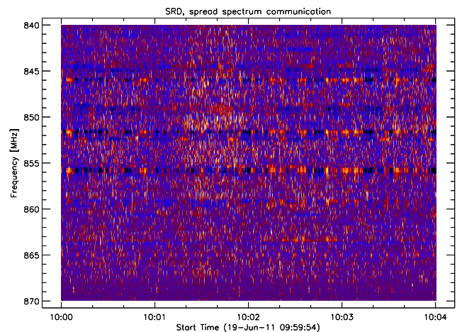
Fig. 39. SRD (short range device) band as broad band digital transmission 24h/7d looking like solar decimetric pulsations.
