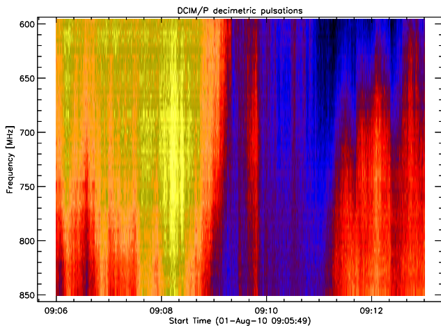
Fig. 10. Decimetric (DCIM) solar radio burst with continuum observed at Bleien observatory, Switzerland. Antenna = 7 m dish, circularly polarized LHCP, pointing to sun.
