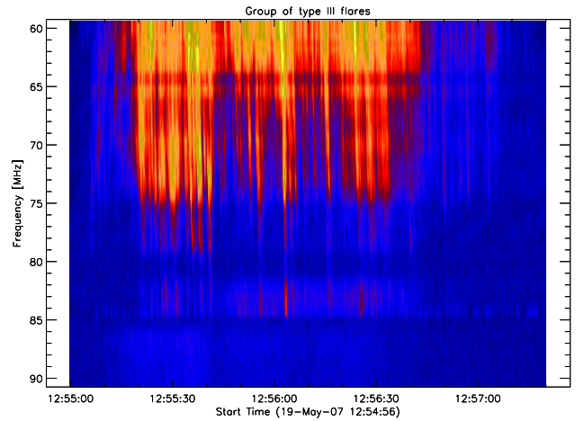
Fig. 5. Group of type III solar radio bursts observed at Bleien observatory, Switzerland. Antenna = log-per CLP-5130, linearly polarized. Some type III are reverse drifting.
