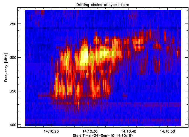
Fig. 1. Noise storm of solar radio emission observed at Bleien observatory, Switzerland. Antenna = dish 7 m, circularly polarized. A chain of type I bursts is shown.
