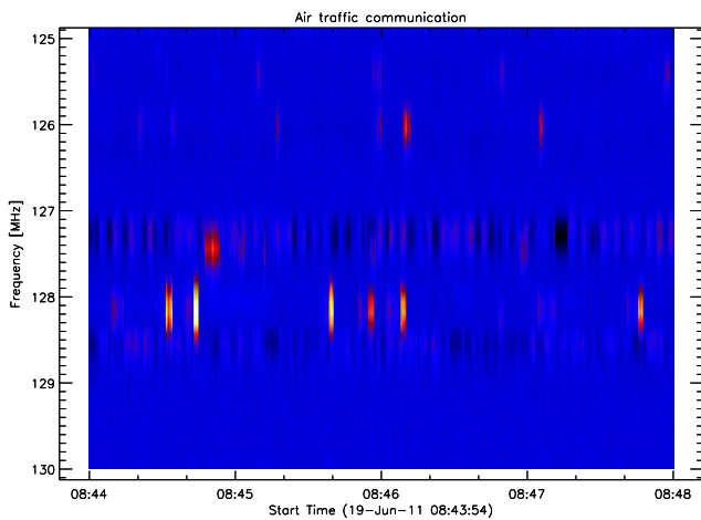
Fig. 29. Sporadic amplitude modulation from air traffic communication.
