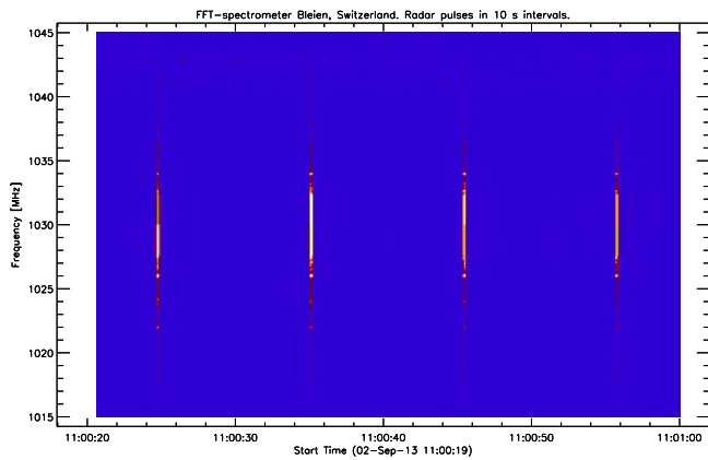
Fig. 43. Reflected radar pulse in the L-band at 1030 MHz observed at Bleien observatory Switzerland.
