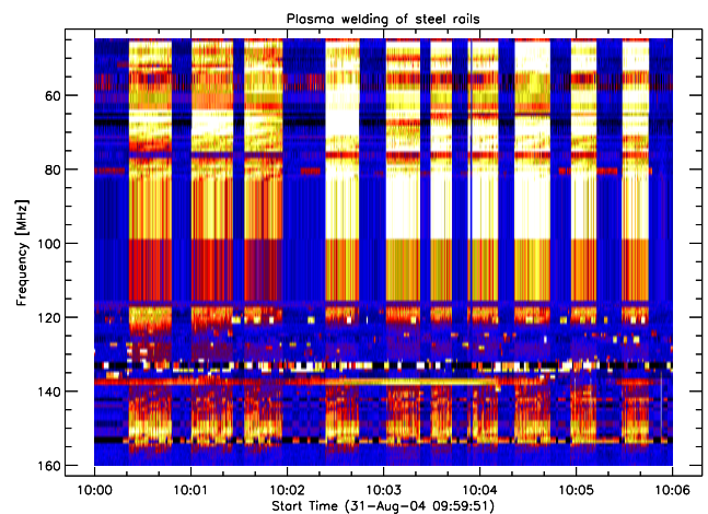
Fig. 19. Interference due to manual plasma welding near the telescope observed at Bleien observatory, Switzerland. Antenna = log-per CLP-5130, linearly polarized 45^\circ .
