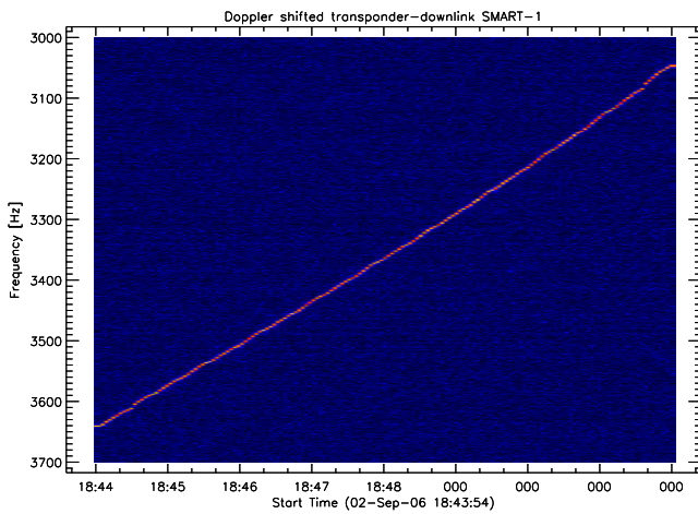
Fig. 24. Weak transponder signal from SMART-1 in its per-lunar orbit. Antenna = 5 m dish, linearly polarized.
