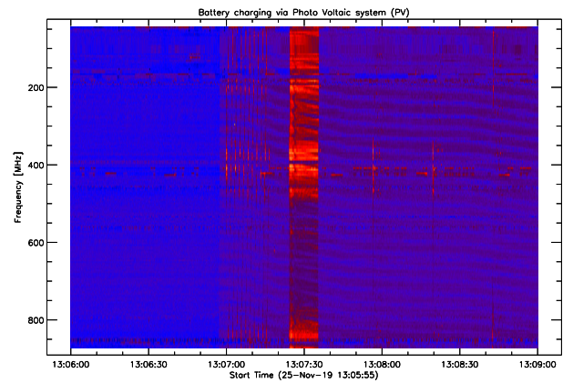
Fig. 61. Interference due to nearby photo voltaic power plant.
