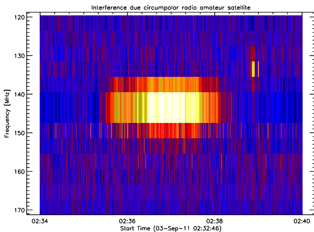
Fig. 40. Fast moving radio amateur (HAM) satellite in the 2 m VHF-band observed in Mauritius.
