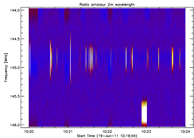
Fig. 30. Sporadic narrow frequency modulation (NFM) from amateur radio communication (HAM) in 2 m band.
