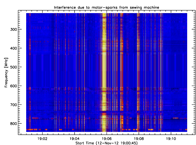
Fig. 53. Strong rfi produced by badly filtered sewing machine.
