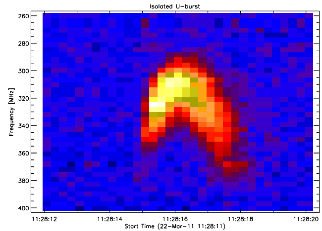
Fig. 13. U-burst in intensity (LHCP+RHCP). Antenna = 7 m dish at Bleien observatory, circular polarized, pointing to the Sun.
