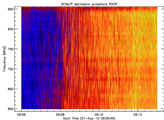
Fig. 9. DCIM (decimetric) solar radio burst with pulsations observed at Bleien observatory, Switzerland. Antenna = 7 m dish, circularly polarized RHCP, pointing to sun.
