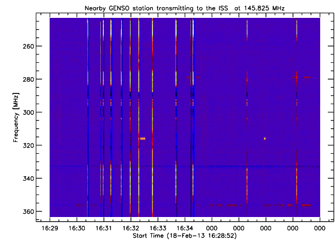
Fig. 31. Sporadic harmonics/cross-talk from strong amateur radio communication (GENSO) in 2 m band.
