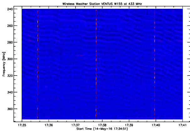
Fig. 55. Interference introduced by a badly designed nearby wireless weather station.
