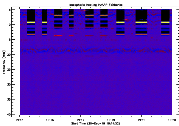
Fig. 59. Interference due to ionospheric heating at HAARP site in Fairbanks.
