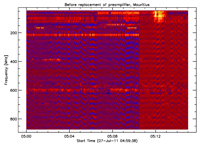
Fig. 22. Interference due to damaged pre-amplifier in the front-end of the telescope observed at MRT observatory, Mauritius. Antenna = large log-per, linearly polarized pointing to sky. Type III solar flare top right with about 30 sfu (300'000 Jansky).
