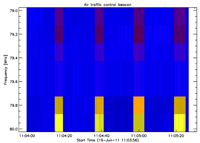
Fig. 27. Beacon of local airport used for radio-navigation. Period about 20 seconds with high transmission power.
