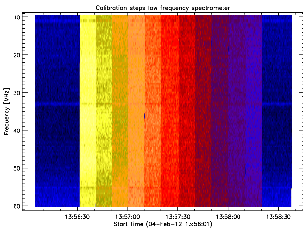
Fig. 48. Calibration steps generated by an adjustable attenuator from 0 dB in steps of 1 dB up to 10 dB) applied to low frequency Callisto. Intensity bars yellow=hot, red=warm and blue=cold.
